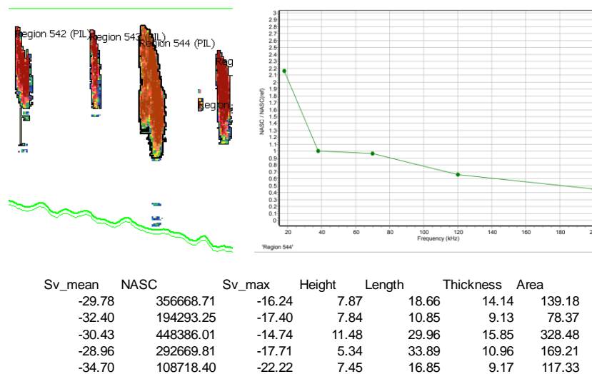
Figure 6. Echogram showing several echotraces attributed to sardine
