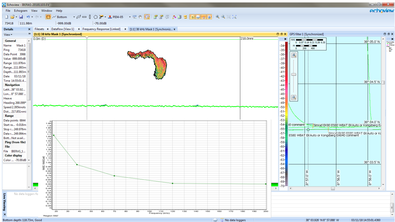
Figure 4. Cleaned echogram showing an isolated echotrace attributed to boarfish I and its characteristic frequency response
